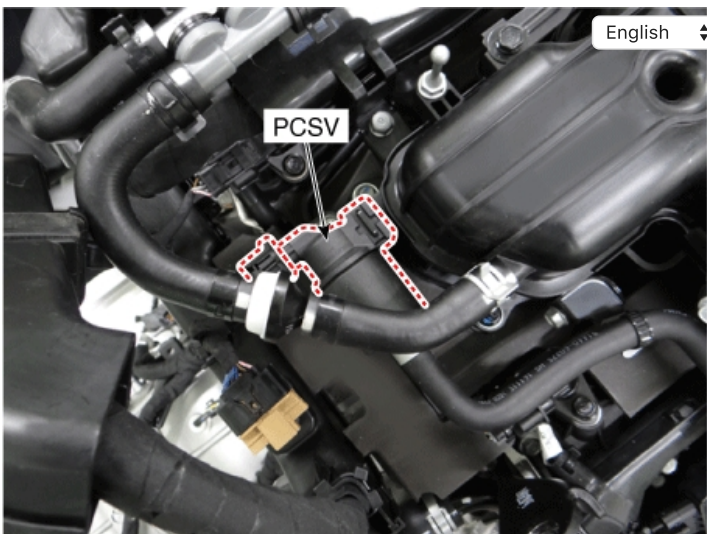
30. CVVT Oil Control Valve (OCV) [Bank 1 / Exhaust]
